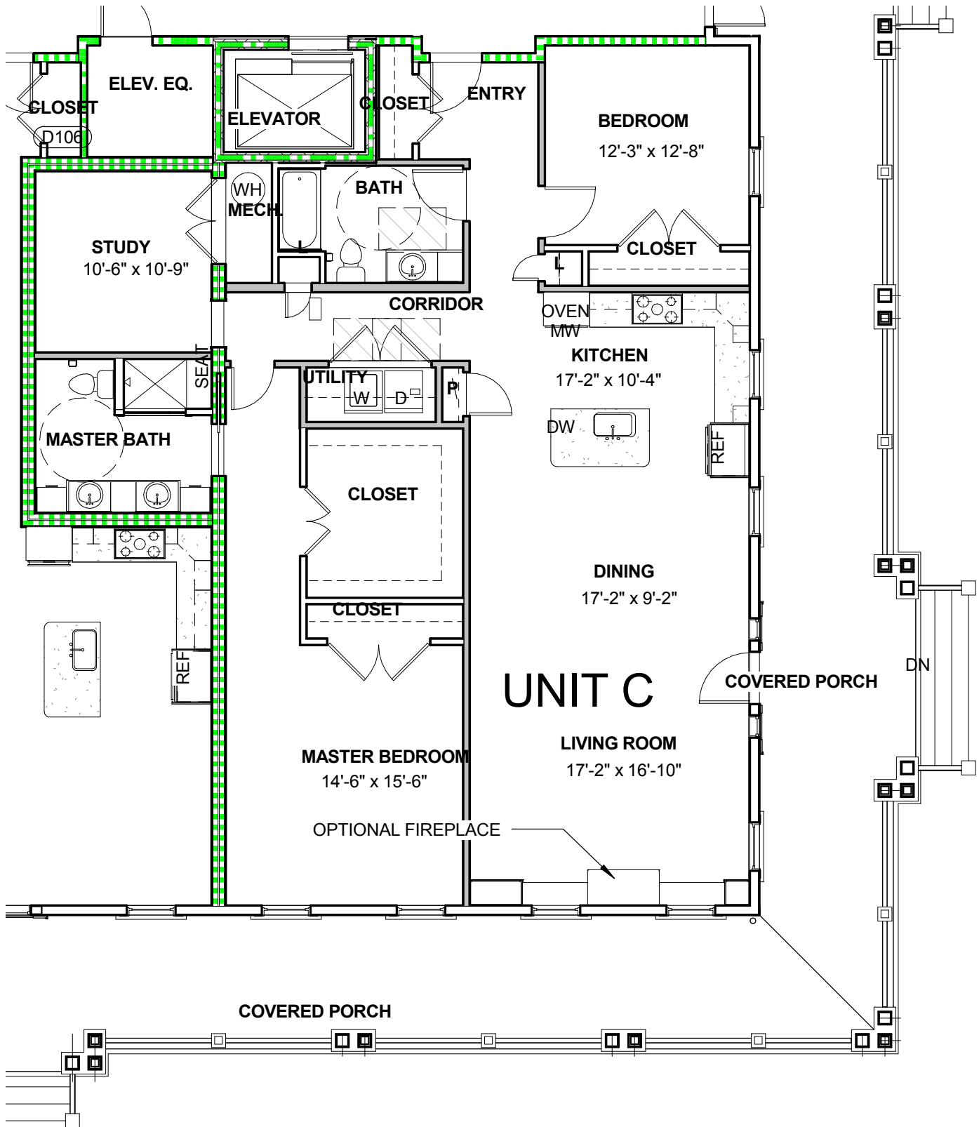
1 LEVEL 01 FLOOR PLAN - UNIT C 1/8" = 1'-0"
